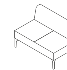
SYM2NA Symbol 2 Seater no arms mm W1020 D690 H685 Seat 410 inch W40 D27 H27 Seat 16
