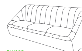
FIJI3SF Fiji 3 seat sofa mm W 2250 D 865 H 885 Seat 470 inch W 88.5 D 34 H 35 Seat 18.5
