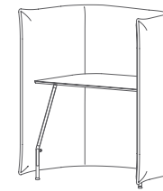
CLODP15H Cloud 1.5 Desk with High Plain Back mm W 1100 D 750 H 1300 Table height 750 inch W 43.5 D 29.5 H 51 Table height 29.5
