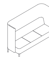
PUL3H Pullman 3 Seat Sofa with Legs mm W 1900 D 675 H 1300 Seat 450 inch W 75 D 26.5 H 51 Seat 18
