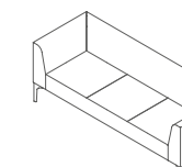
SYM32A Symbol 3 Seater 2 arms mm W1890 D690 H685 Seat 410 inch W74.5 D27 H27 Seat 16
