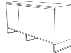
SB16 Sideboard 1600 mm W 1600 D 500 H 750 inch W 63 D 19.5 H 29.5
